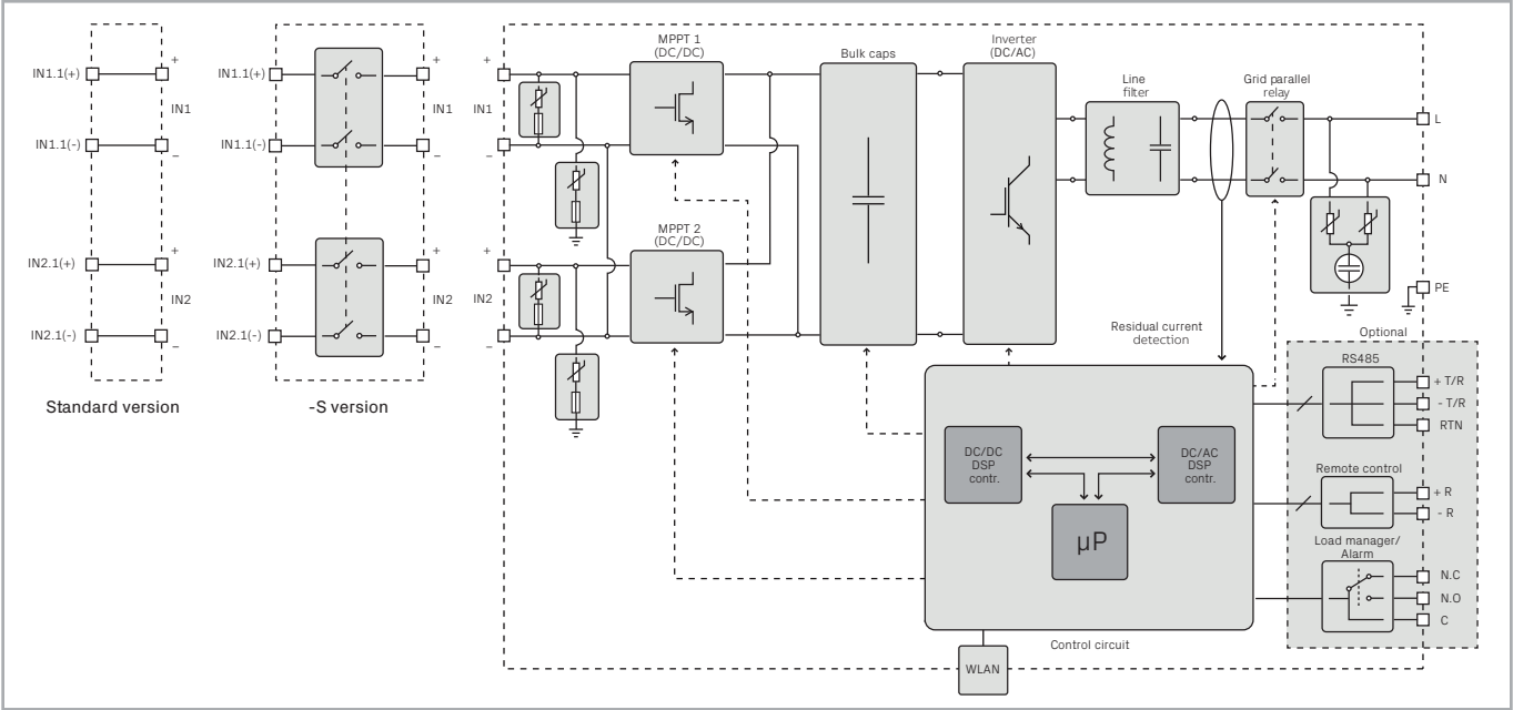
UNO-DM-3.3/4.0/4.6/5.0-TL-PLUS-Q string inverter block diagram
