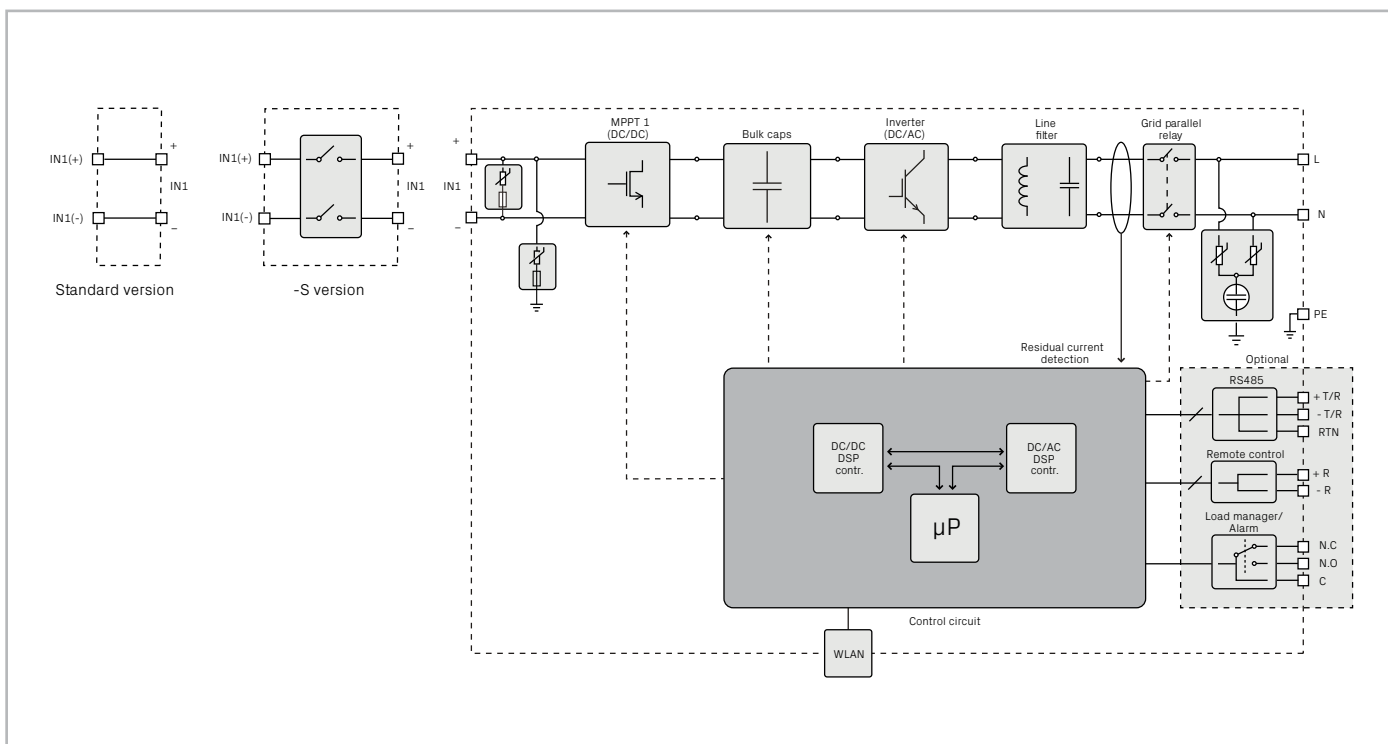
UNO-DM-1.2/2.0/3.0-TL-PLUS-Q string inverter block diagram
