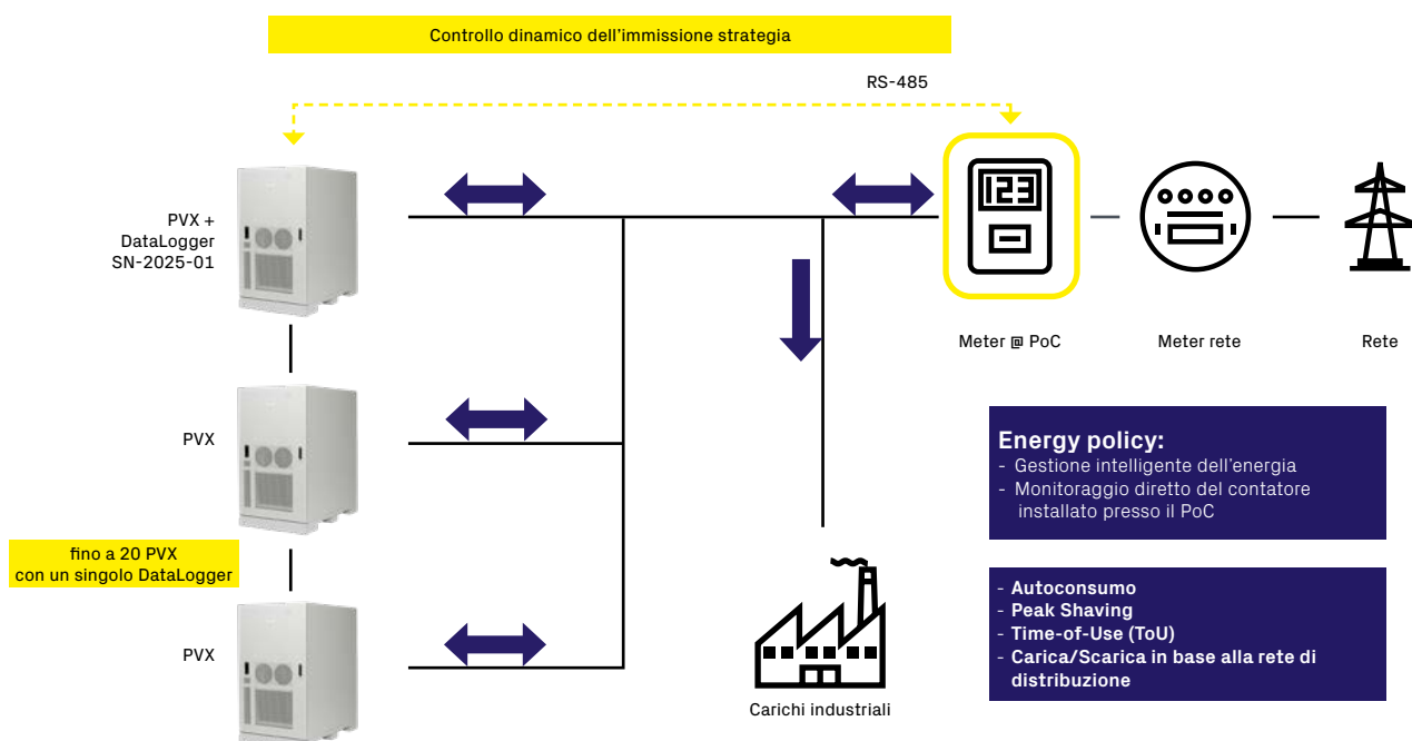
FIMER PVX-241.0
